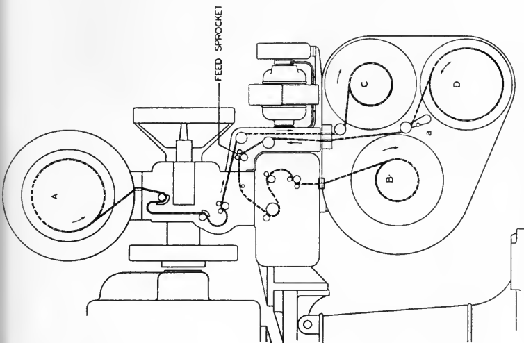
FIG. 2. Film path through projector.
